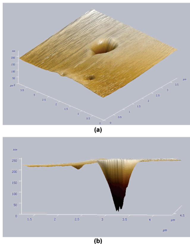
Figure 6. At 2 mN nanoindentation of the film surface (here shown for the SiMe25 sample) with deep tip penetration masks the measurements due to the effect of the substrate. (a) and (b) show two different views.
