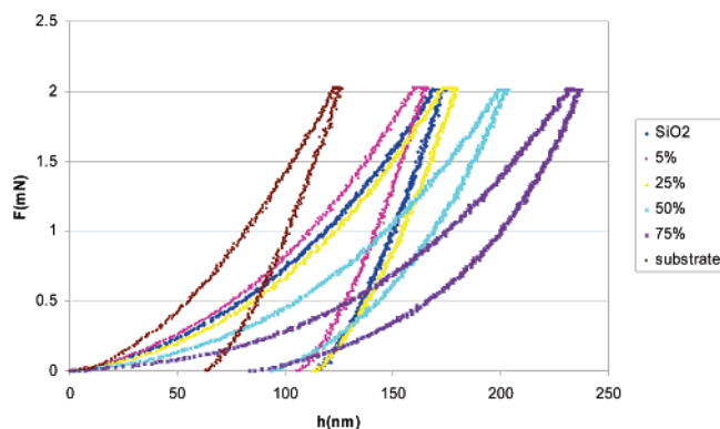
Figure 2. Loading curves for ORMOSIL thin films with varying degree of alkylation of the silica matrix.
