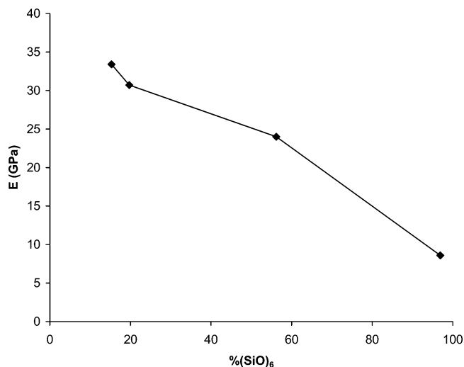
Figure 10. Correlation between the elastic modulus and the percentage of (\text{SiO})_6 rings in the organosilica matrix.
