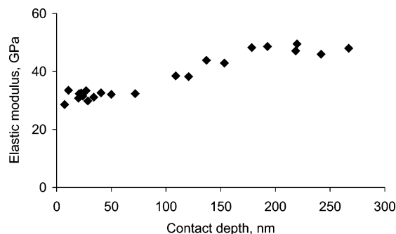
Figure 5. Variation of the elastic modulus versus contact depth for the Si5Me film.
