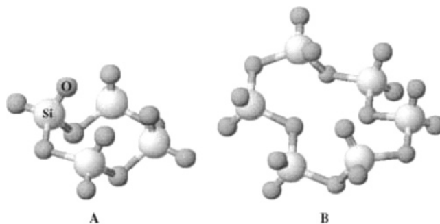
Figure 9. Schematic diagram of the more common types of primary cyclic arrangements of the structural units, \text{SiO}_4 , in xerogels: (A) four-membered siloxane ring (\text{SiO})_4 and (B) six-membered siloxane ring (\text{SiO})_6 .
