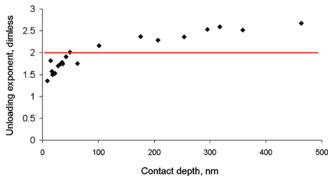
Figure 7. Variation of the unloading exponent ( b ) versus contact depth.
