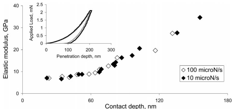
Figure 3. Elastic modulus of the Si100Me film undergoing nanoindentation at different speeds and, in the inset, loading curves for the Si50Me film at different speeds (black line, 7 mN/s; gray line, 70 mN/s).
