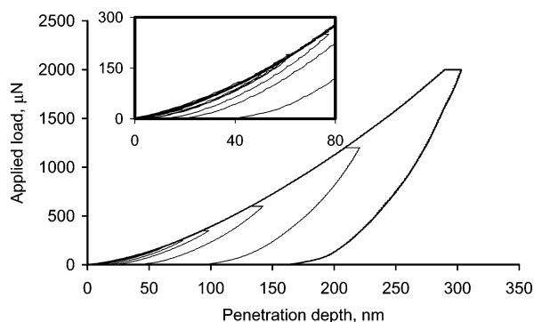
Figure 4. Loading-unloading force curves at varying loads between 30 and 2000 \mu\text{N} for the Si50Me film.
