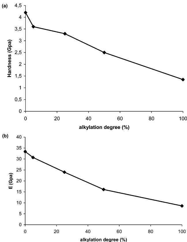
Figure 8. Hardness (a) and elastic modulus (b) as a function of the degree of alkylation of the silica matrix in ORMOSIL thin films.
